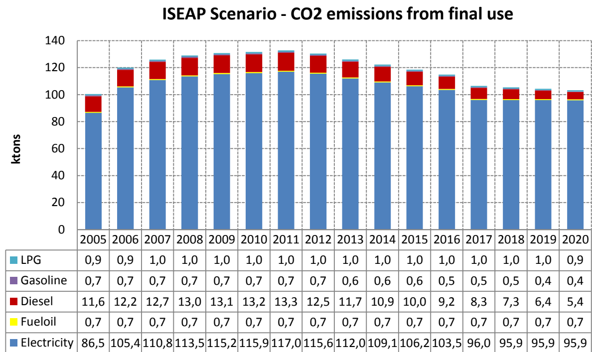
Figure 3.51. ISEAP Scenario – Growth trend of CO 2 emissions from final use per energy carrier
